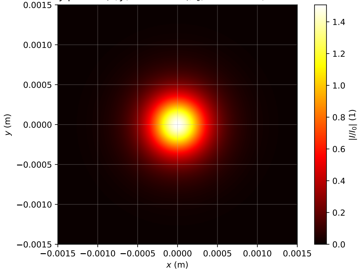
Intensity profile I(x, y, z = 1.274m)/I_0 , Pin=0.9Pcr, artificial time
